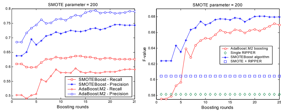
Fig. 3. Precision, Recall, and F-values for the minority class when the SMOTEBoost algorithm is applied on the Mammography data set
