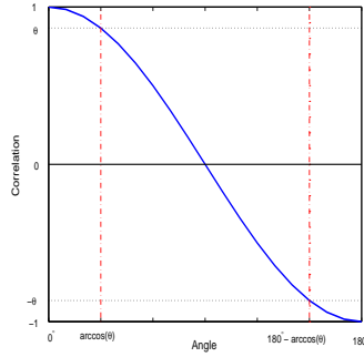
Fig. 2. Cosine Value vs. Central Angle
