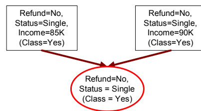
(b) Specific-to-general
