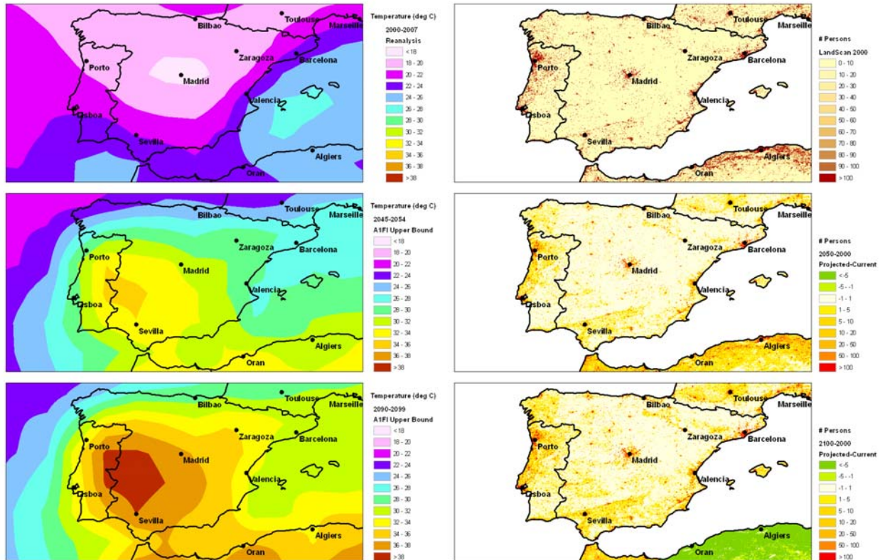
Figure 5. Observed and Projected Extreme Heat Events (Upper Bound Only) and Population in Spain
