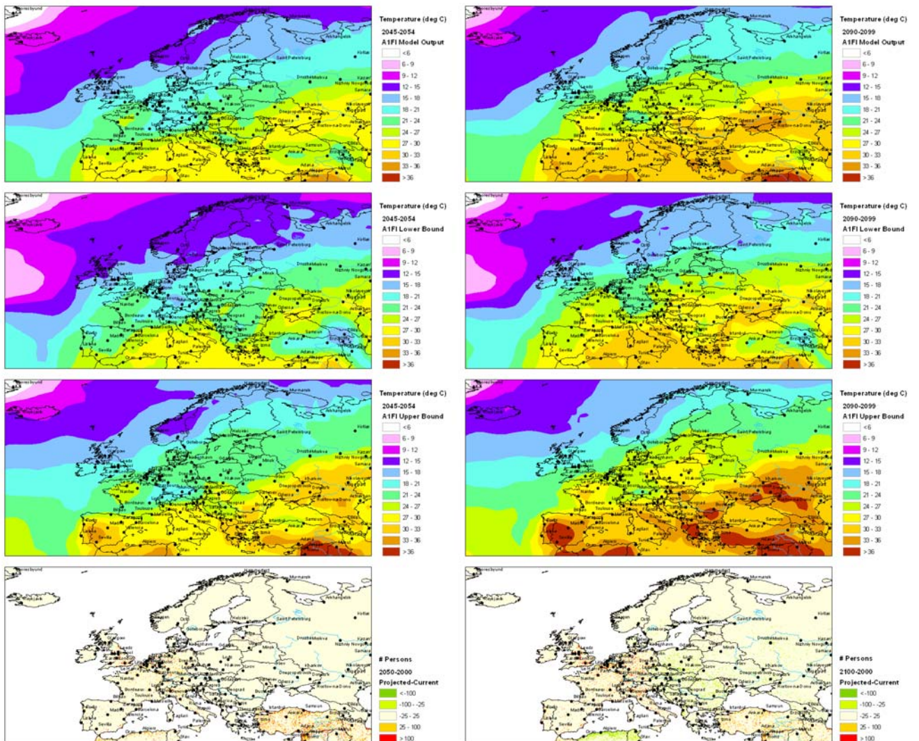
Figure 4. Projected Extreme Heat Events and Population for the Middle and End of the 21 st Century in Europe
