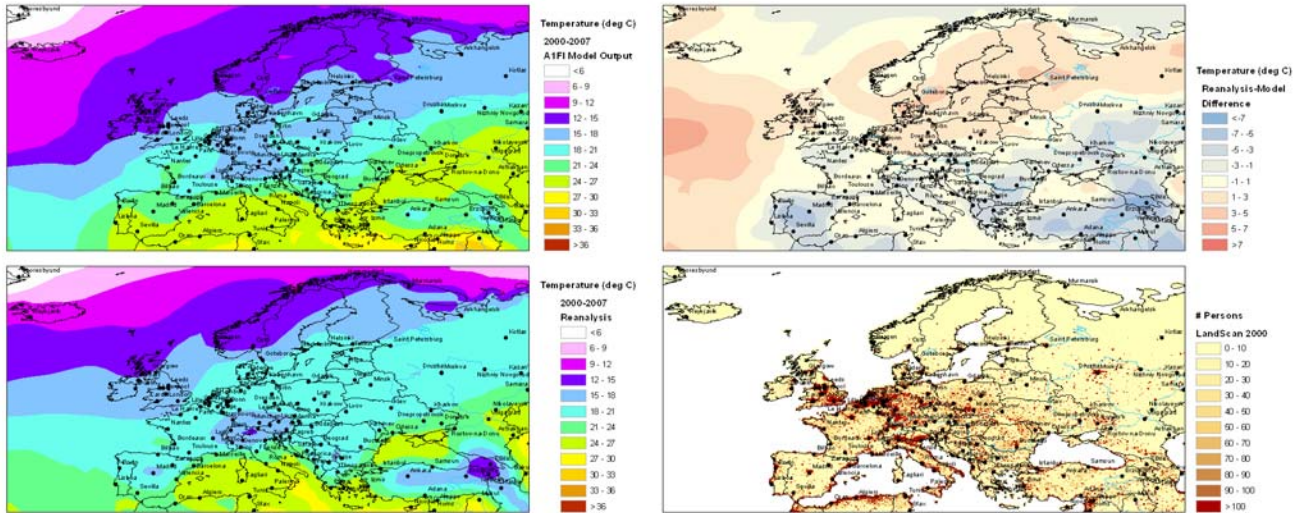
Figure 3. Model vs. Observed Extreme Heat Events and Population for the Present Time (2000-2007) in Europe
