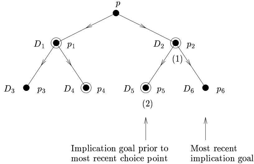
Figure 5.1: Example of an Implication Tree
