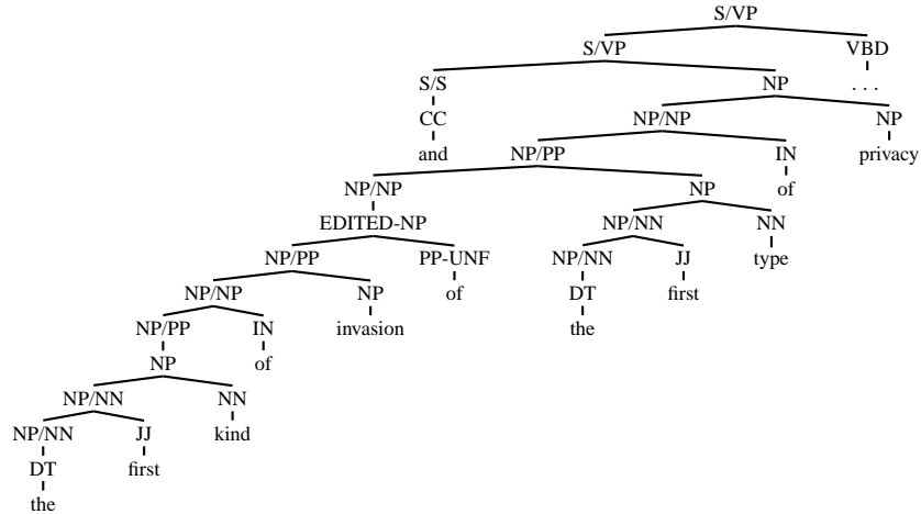
Figure 2: Right-corner transformed tree with repair structure
