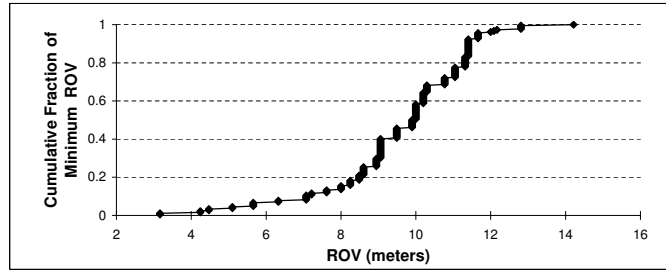
Fig. 13. ROV enforcement results. This graph is generated using a real deployment of 200 XSN nodes. For a ROV of 10 meters, the average minimum distance between sentry pairs is 9.57m with a standard deviation of 1.88m.
