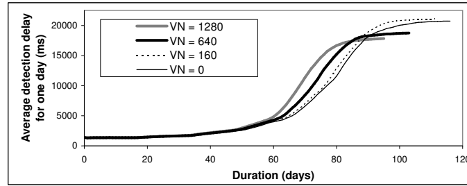
Fig. 25. Influence of number of targets per day (VN) on average detection delay (ADD).
