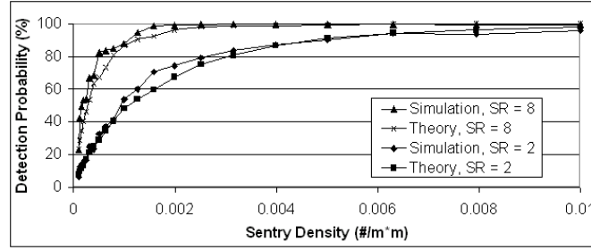
Fig. 35. Comparison Between Theory and Simulation: Detection Probability Versus Sentry Density When Using the Sentry Service. For a sensing range of 2m, the Pearson Correlation Coefficient (R) between theory and simulation equals 0.994. For a sensing range of 8m, R=0.984.
