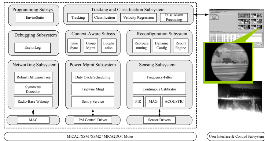
Fig. 9. The VigilNet system architecture. The three power management services described in this paper can run on a XSM node along with additional power management techniques (e.g., robust diffusion tree), context-aware services (time synchronization, group management, localization), reconfiguration subsystems (reprogramming, reconfiguration, reporting), and tracking and classification subsystems.
