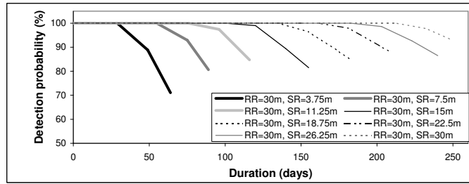
Fig. 32. Influence of sensing radius (SR) on detection probability (DP).
