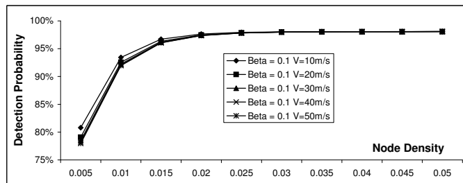
Fig. 7. Effect of sentry density (in number of nodes per m^2 ) on detection probability, according to wakening period ratio \beta and target velocity. This graph is generated using a theoretical model. The target velocity does not noticeably impact the detection probability when node density is reasonably high.
