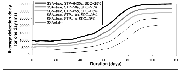
Fig. 19. Influence of sentry toggle period (STP) on average detection delay (ADD).
