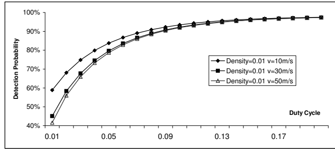
Fig. 6. Effect of sentry duty cycle (SDC, in % / 100) on detection probability according to node density (in number of nodes per m^2 ) and target velocity. This graph is generated using a theoretical model. A high detection probability can be achieved even with a relatively low duty cycle.
