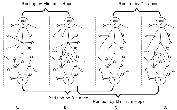
Fig. 1. Four different ways of implementing the tripwire service. For routing purposes, the tripwire service can either use the route with the minimum number of hops, or the route with smallest physical distance. The tripwire partitions can be determined using either the distance to the base or the minimum number of hops to the base.
