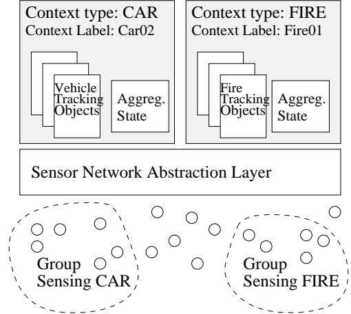
Figure 2. Programming model
