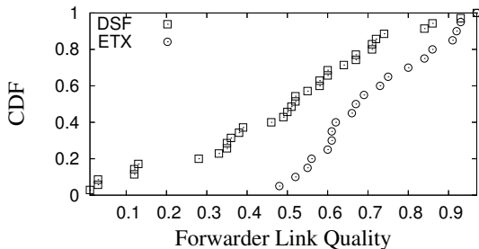
Fig. 18. Diversity in Forwarder Link Qualities
