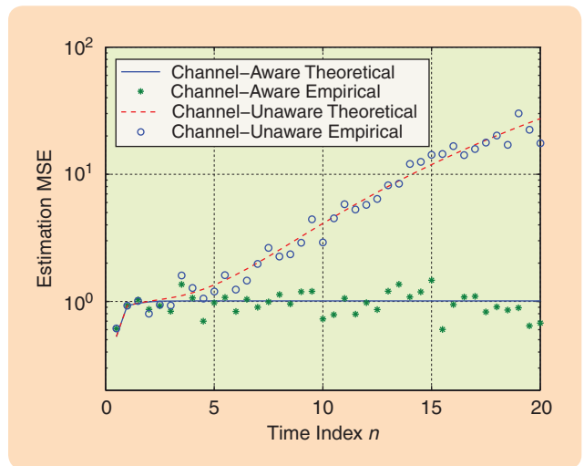
FIGURE 15 Estimated mean-squared error at the fusion center versus time n . The setting involves a wireless sensor network with K = 50 sensors and each sensor acquiring M_k = 10 temperature measurements. The temperature evolves according to a zero-acceleration propagation model. Each sensor reduces the dimensionality of \tilde{\mathbf{y}}_k(n|n-1) to l_k = 1 , and transmits these scalars over noisy links to the fusion center.
