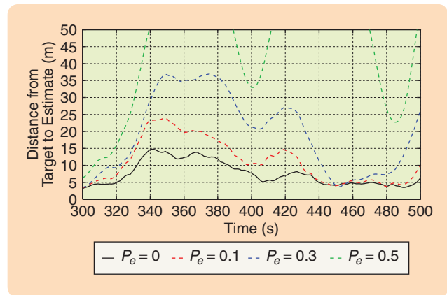
FIGURE 7 Effect of packet errors on the extended sign of innovations Kalman filter (SOI-KF). The root-mean-squared error (RMSE) of the extended SOI-KF for the target-tracking problem of Figure 4 is shown when packets are lost with probabilities P_e = 0 , P_e = 0.1 , P_e = 0.3 , and P_e = 0.5 . Errors in packet decoding cause the predicted observations \hat{y}(n|\mathbf{m}_{0,n-1}) to drift across different sensors, which results in an inconsistency between the sign of innovations m(n) computed at the sensor scheduled for transmission and its interpretation by receivers. This effect is not catastrophic if the drift of the predicted observations \hat{y}(n|\mathbf{m}_{0,n-1}) is small compared with the observation noise variance \sigma_v(n) . For the simulation parameters of Figure 4, the filter's RMSE performance degrades smoothly for P_e = 0.1 and P_e = 0.3 . For P_e = 0.5 the RMSE error increases beyond acceptable levels.
