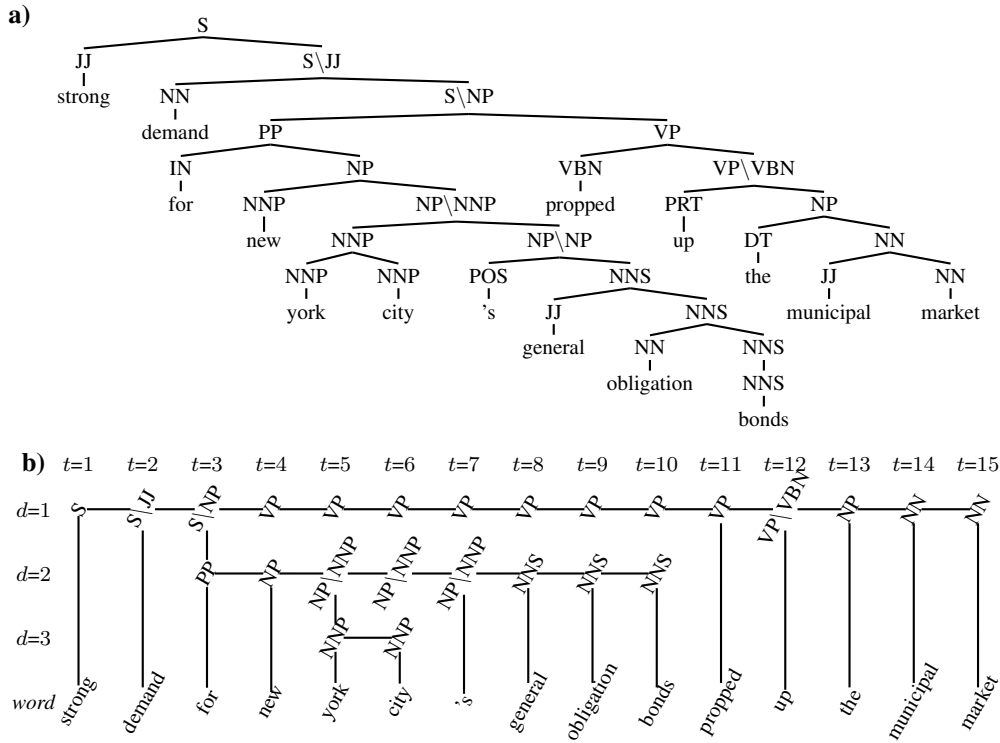
Figure 4 A left-corner transformed version of the tree and memory store from Figures 2 and 3.
