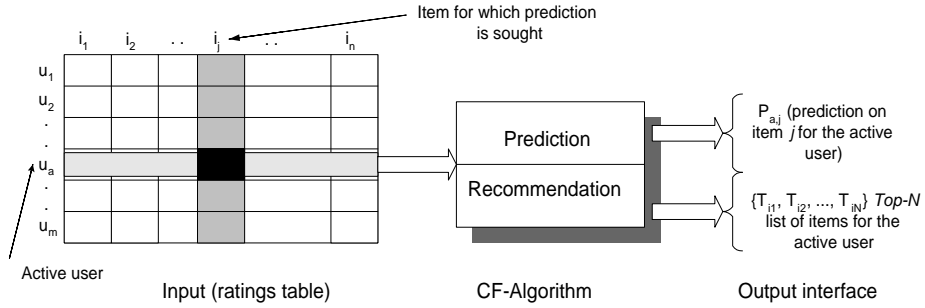
Figure 1: The Collaborative Filtering Process.
