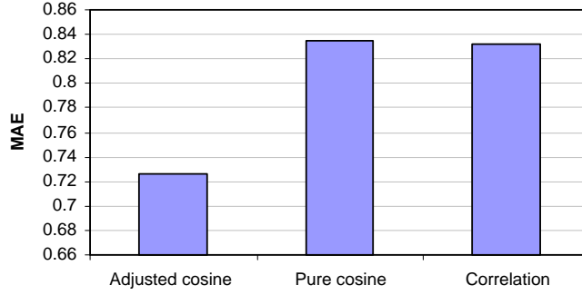
Relative performance of different similarity measures
