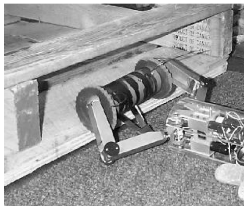
Fig. 5. TerminatorBot placing a Scout onto a platform for surveillance. The Scout is incapable of rolling or hopping onto the platform but can roll itself to the platform. The TerminatorBot cannot carry things while locomoting, but it can crawl up behind them for assistance. This demonstrates how TerminatorBot and Scout can cooperate as part of a heterogeneous system.
