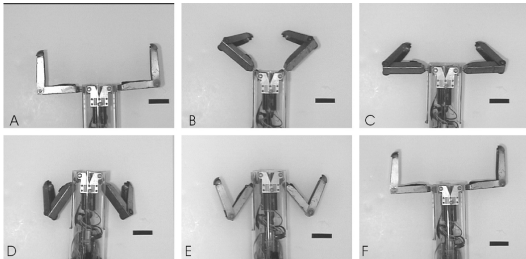
Fig. 6. TerminatorBot locomoting using a swimming gait. (a), (f) Shows a starting point to reference forward motion using the black line. (b) The arms are positioned forward of the body and rotated down to lift off the ground. The arms are rotated back while on the ground, driving the body forward, as shown in (b)–(d). The arms are lifted off the ground (e) for repositioning to start the next gait cycle.
