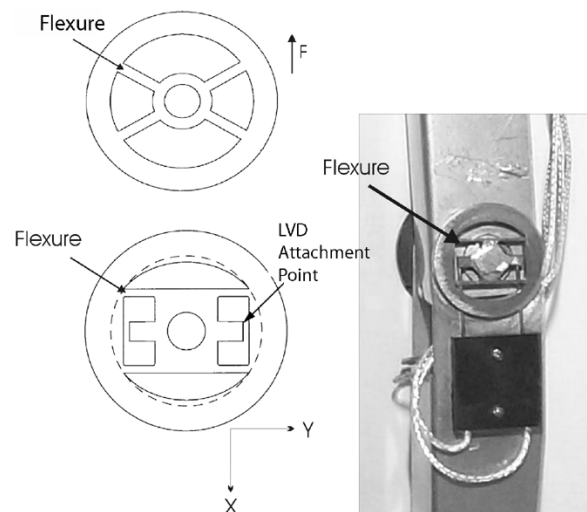
Fig. 3. (Top left) Traditional torque sensor, which has a tendency for torques to saturate the sensor more easily than forces. (Bottom left) Torque sensor with biased flexures, for equalizing force and torque sensitivities. (Right) Specialized sensor attached to the elbow of TerminatorBot.
