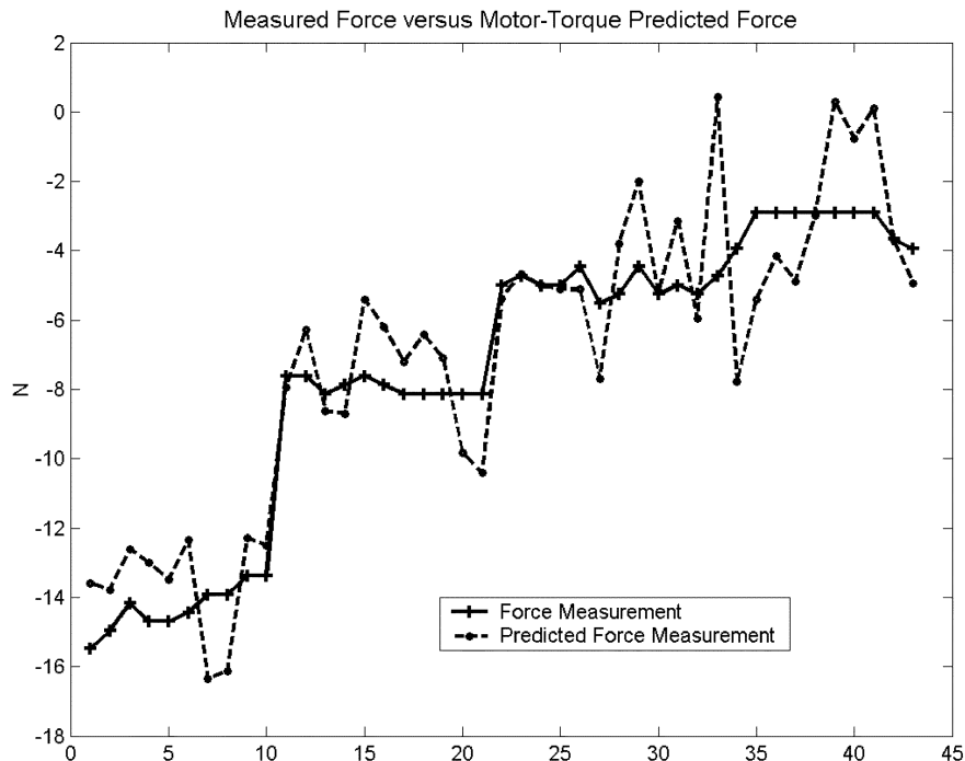
Fig. 2. Plot of actual versus predicted force measurements using motor encoders. Predictions were based on motor torque values generated in closed-loop control. Actual measurements were taken from a Lord force/torque sensor.
