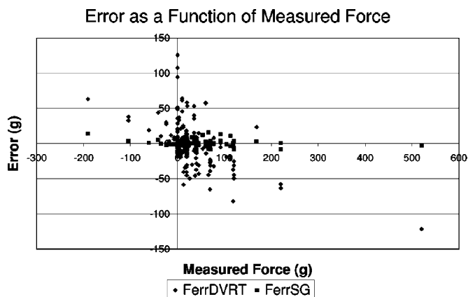
Fig. 4. Plot of calibrations for our force/torque sensor using strain gages and DVRTs. Strain gages outperformed DVRTs. Strain gage error in measurement is on the scale of 20 g, versus 100 g for the DVRTs. Strain gages also show a trend of decreased error as applied force increases.
