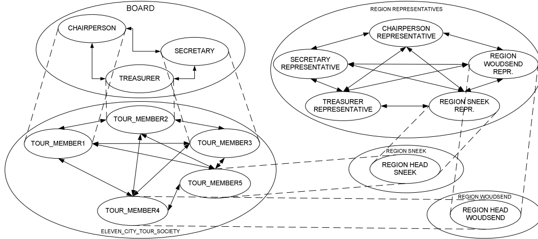
Fig. 9. Eleven cities tour organization after formation of the Regions and Region Representatives groups.
