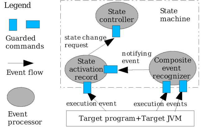
Figure 3: The components for a state machine.
