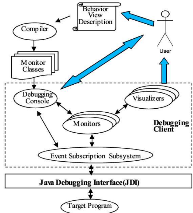
Figure 2: The architecture of the scenario-driven debugger.
