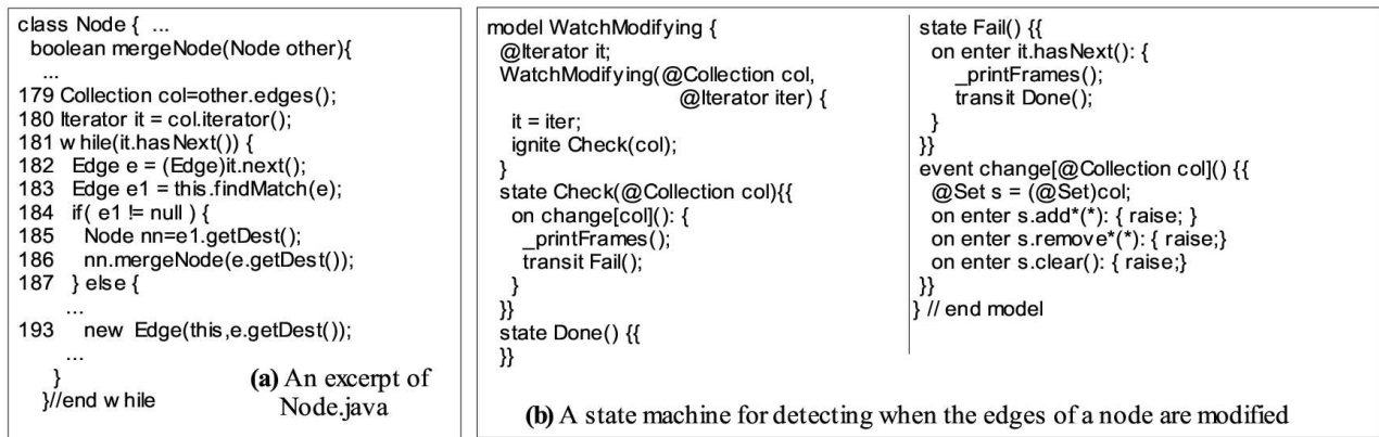
Figure 6: Investigating Bug 1 with a behavior view.
