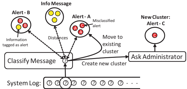
Fig. 5. Overview of classification methodology
