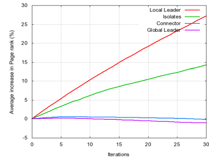
Figure 4: Change in Average Page Rank with our recommendation model compared to document similarity model.
