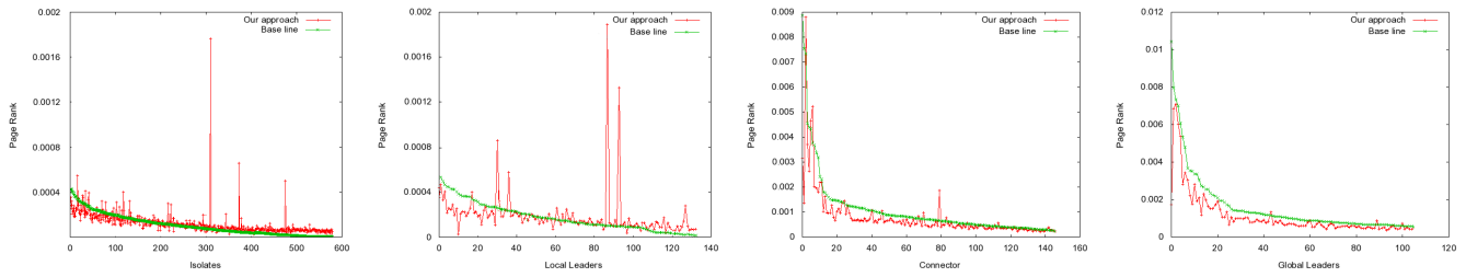
Figure 3: Category wise change in the page rank of bloggers after using our recommendation algorithm.
