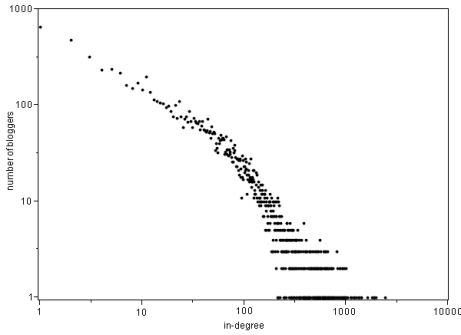
Figure 1: Log-Log plot of degree distribution of core nodes.
