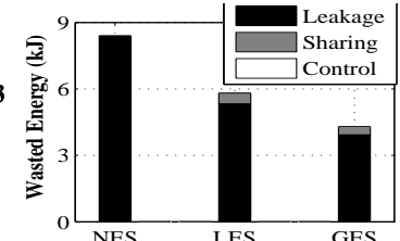
(b) Wasted Energy Comparison
