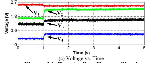
Figure 16. Two-to-One Energy Sharing
