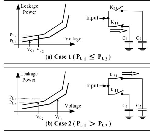
Figure 7. Charging Control Example
