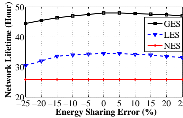
(b) Impact of Energy Sharing Error
