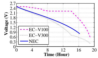
(c) Capacitor Voltage vs. Time
