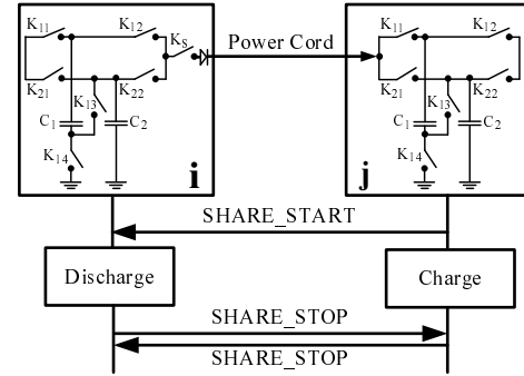
Figure 9. Energy Access Protocol
