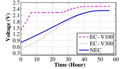
(c) Capacitor Voltage vs. Time
