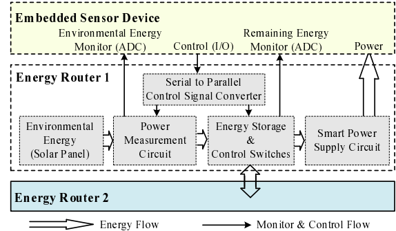
Figure 4. Energy Router Hardware Architecture
