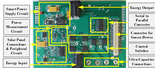
Figure 5. Energy Router Platform
