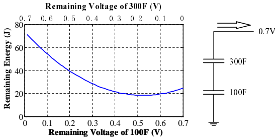
Figure 8. Different Voltage Combinations
