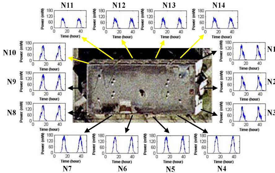
Figure 17. Experiment Site & Harvested Power Distribution
