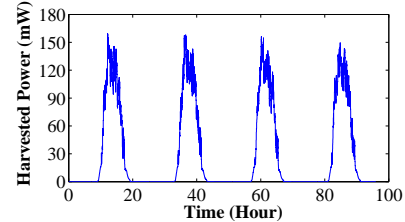
Figure 14. Harvested Power Over 4 Days
