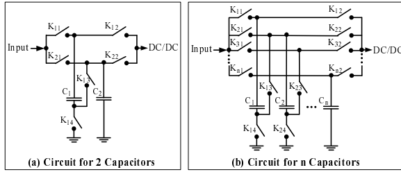
Figure 3. Capacitor Array Circuit
