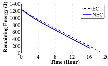
(b) Remaining Energy vs. Time
