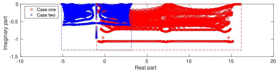
FIG. 3.1. Comparison of the spectrum between Case one (1.2) and Case two (3.1). The test matrix is based on finite difference method on a 100^2 grid, with absorbing layers near the boundary. The eigenvalues are computed by eig in MATLAB. The rectangles are the results of Lemma 3.1 and Theorem 3.2, where \rho_1 \approx 17.2 , \rho_2 \approx 1.3 .
