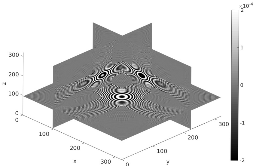
FIG. 7.2. Solution of the problem in Figure 7.1.
