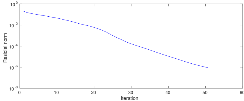
FIG. 8.3. Residual history of FCI iterations of SEG/EAGE salt-dome model.
