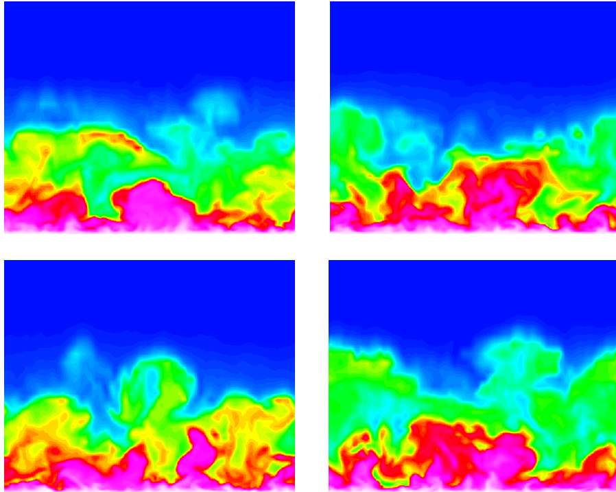
Figure 5. Example of “bursting” shown in spanwise planes from the Mach 4.0 adiabatic wall boundary layer simulation of Martin & Candler [MC00].
