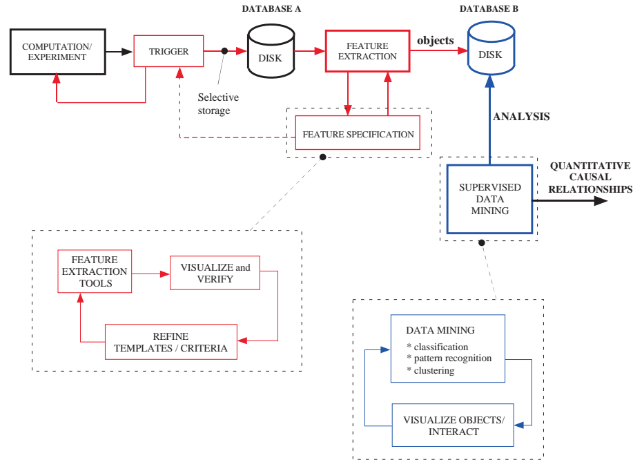
Figure 3. Schematic of our new data analysis approach. The connected boxes enclosed by dotted lines are essentially the same, with the larger boxes showing the internal features of the smaller ones, and have been drawn separately for clarity.
