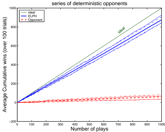
Figure 2: ELPH accumulated wins over time against a synthetic agent playing from a non-stationary set of randomly selected deterministic policies. Results are for 100 trials of 1000 plays.
