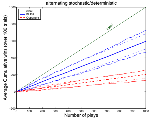
Figure 4: ELPH accumulated wins over time as in Fig. 3, but with \lambda = 0, 1 chosen randomly, each with probability 1/2. Results shown for 100 trials of 1000 plays.
