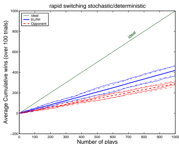
Figure 5: ELPH accumulated wins over time as in Fig. 4 except that each policy was played for a randomly selected time chosen from a Poisson distribution with \mu = 3 . Results shown for 100 trials of 1000 plays.
