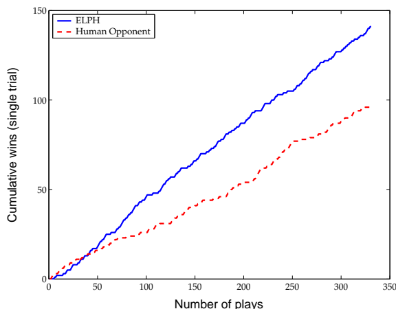
Figure 6: ELPH accumulated wins over time against a human opponent. Results shown for a single match.
