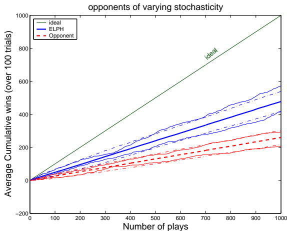
Figure 3: ELPH accumulated wins over time against a synthetic agent that plays from a non-stationary set of stochastic policies of the form (1). Results shown for 100 trials of 1000 plays.
