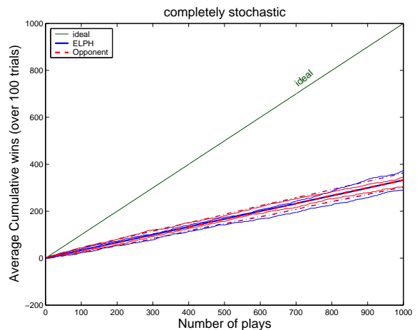
Figure 1: ELPH accumulated wins over time against a stochastic synthetic agent. Results are for 100 trials of 1000 plays. We show the mean and plus/minus twice the standard deviation.
