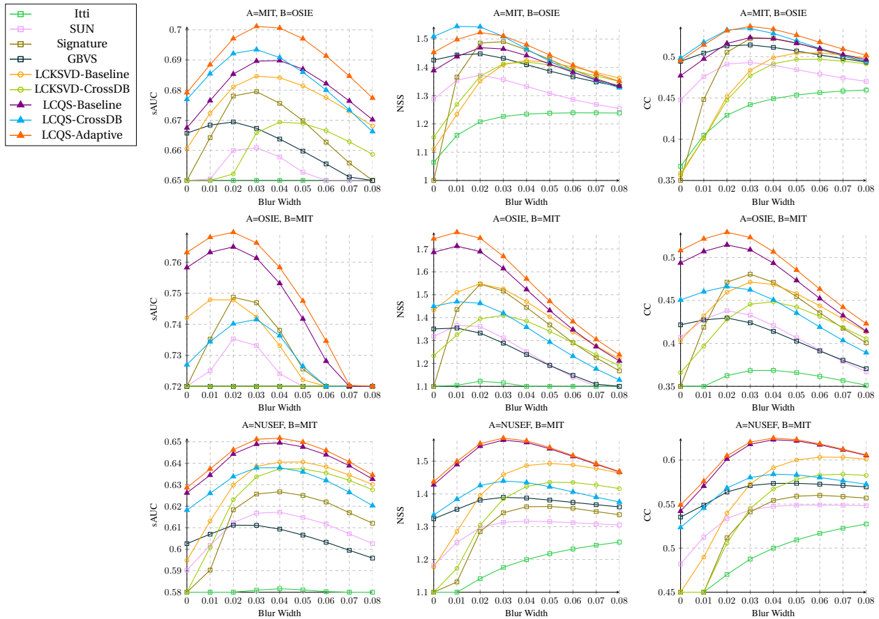
Figure 3: Shuffled AUC, NSS and CC scores on various datasets with various models. The blur width is parameterized by a Gaussian's standard deviation in image widths.
