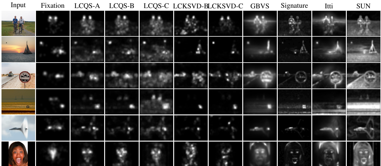
Figure 4: Qualitative results of the proposed LCQS saliency model and various state-of-the-art models. Row 1 & 2 are samples from MIT dataset, Row 3 & 4 are samples from OSIE dataset, and Row 5 & 6 are samples from NUSEF dataset. The configuration for the cross dataset learning are as stated in Section 5.1. The suffix A , B , and C stand for Adaptive, Baseline, and CrossDB, respectively.
