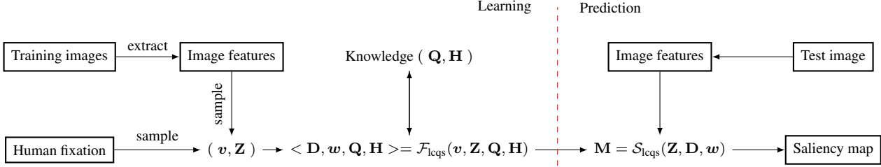
Figure 1: An overview of the LCQS saliency model.
