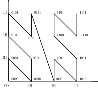
Figure 5: Bit Interleaving in Peano SFC.
