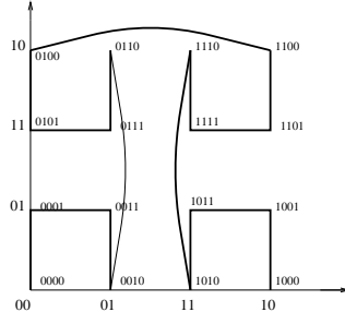
Figure 7: Bit Interleaving in Peano SFC.
